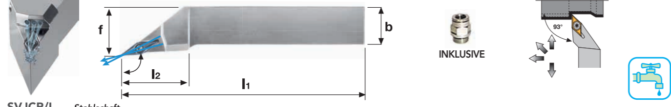
SVJCR/L Stahlschaft
